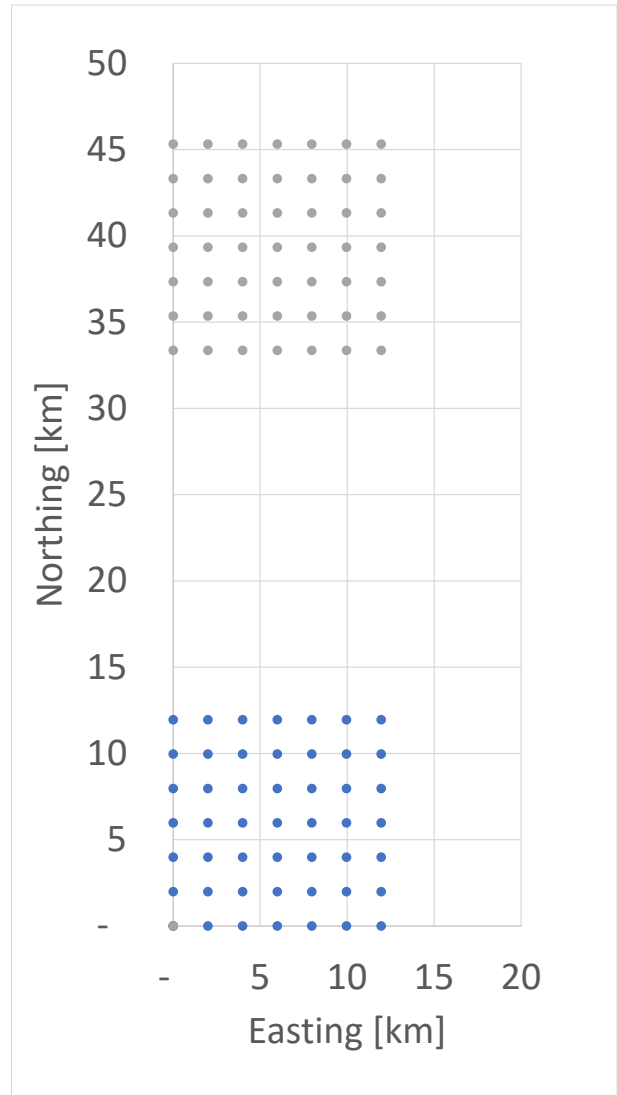
Figure 8: Layout with 7 MW/km 2 build-out density (for each farm) and 21.410 km spacing between farms (run ID 21).
